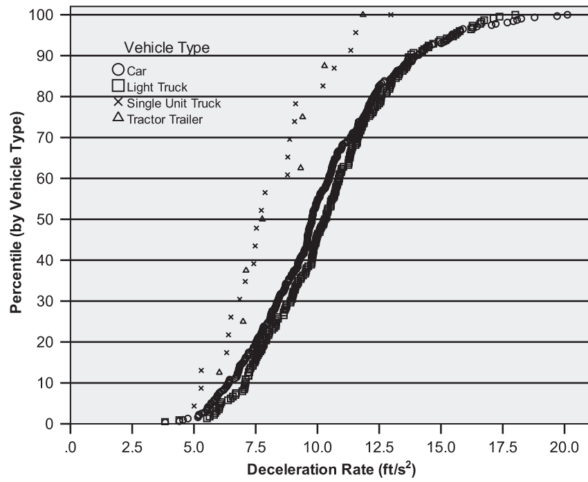
FIGURE 3 Cumulative distribution for deceleration rate by vehicle type.
